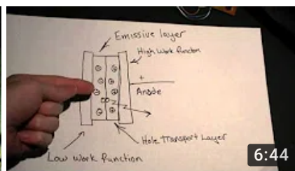
Making an OLED - Light from Carbon Compounds
