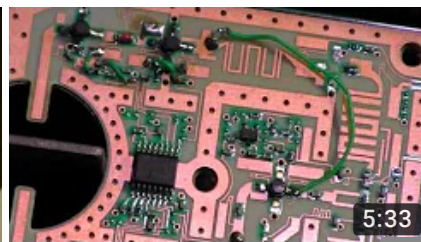
Microwave Handy Scanner - TSA Body Imaging at Home
