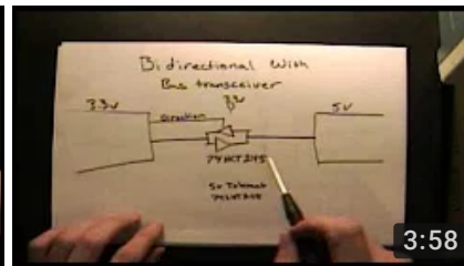
Short Circuits Logic Level Shifting - The Days of 5 Volt...
